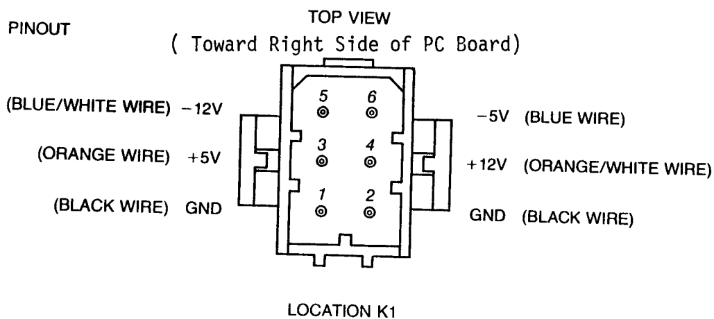
Figure 5 POWER CONNECTOR
